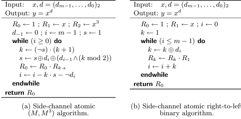
Fig. 4. Further simplified algorithms for constrained devices.
